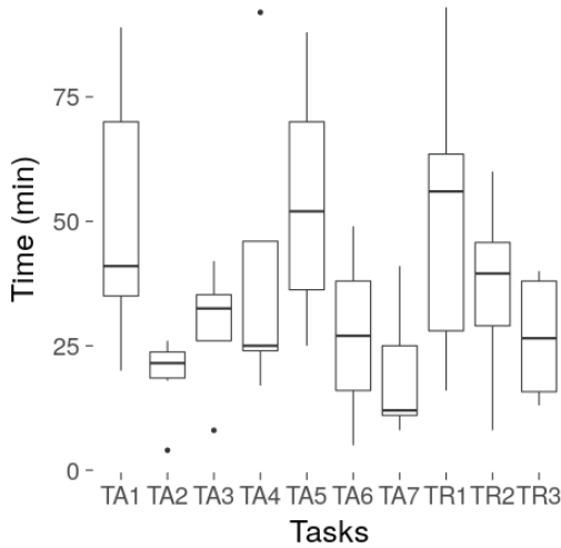
Fig. 2: Time spent per task. Timing includes failed attempts.
